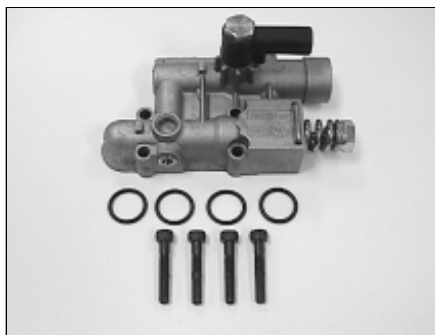
16031 Manifold Assy.
